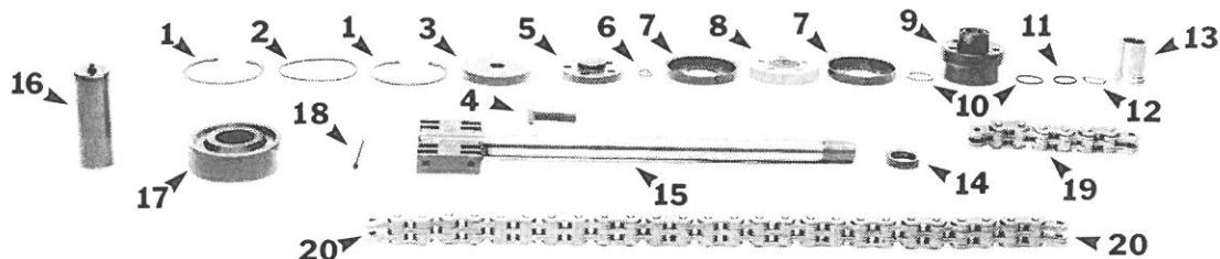
HYDRAULIC LIFT REPLACEMENT PARTS FOR AUBURN TRENCHERS
