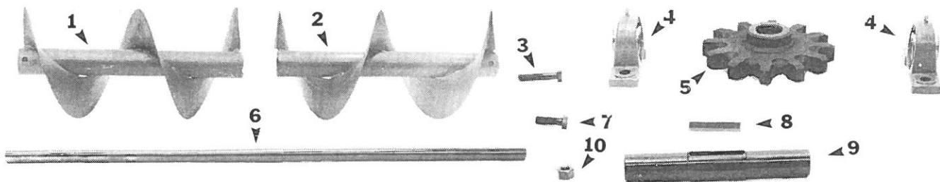
REPLACEMENT AUGER & SHAFT ASSEMBLIES FOR AUBURN TRENCHER
