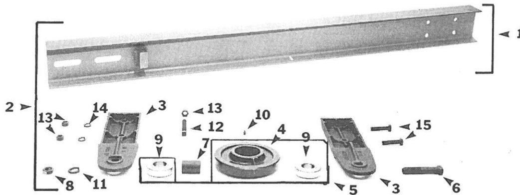
REPLACEMENT BOOM ASSEMBLIES & BOOM PARTS FOR AUBURN TRENCHERS
