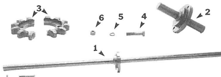
SPECIAL REPLACEMENT AUGER SHAFT & BOLT ON SPLIT SPROCKET
